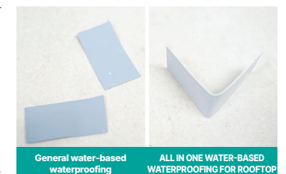
Flexibility test after freezing at -15°C ▶
